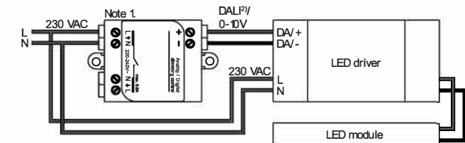
Wiring diagram, directly powered DALI or 0-10V drivers Suitable for drivers that can be switched of via control interface
