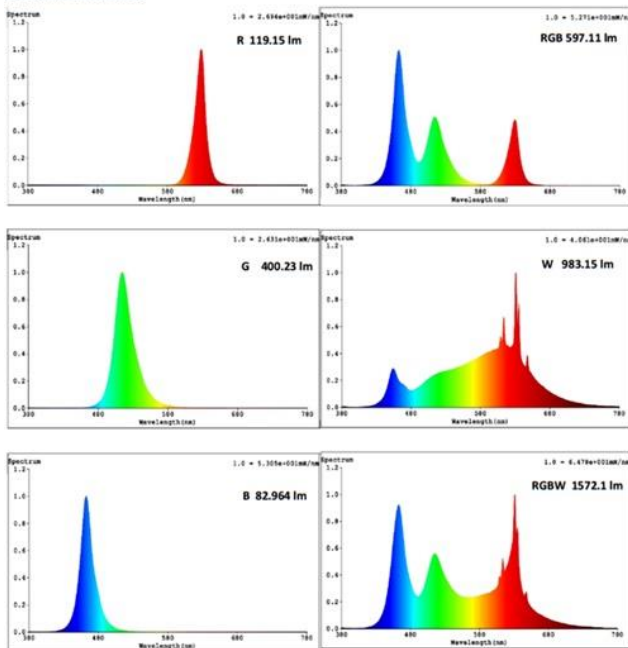
Spectrum Distribution
